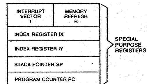
Z80-CPU REGISTER CONFIGURATION
